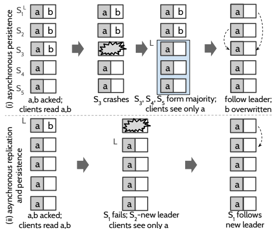
Figure 1: Poor Consistency atop Asynchronous Durability. (i) shows how non-monotonic reads result upon failures with systems that persist asynchronously. (ii) shows the same for systems that replicate and persist asynchronously. Data items shown in grey denote that they are persisted.
